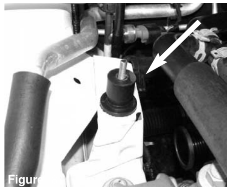
Figure 5 Loosen the clamp on the turbo using 8mm nut driver. Pull the hose away from the turbo housing.
