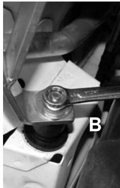
Figure 15 A) Now secure the bracket using provided m6 nut and washer. B) Tighten using 10mm wrench.
