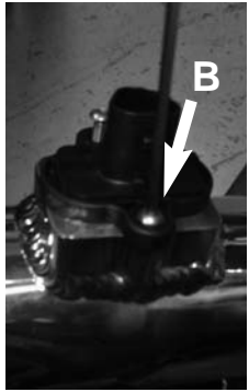
Figure 19 Attach the vibra mount to the hole used to hold in auxiliary inlet. Secure using provided nut and washer and tighten using 10mm wrench.
