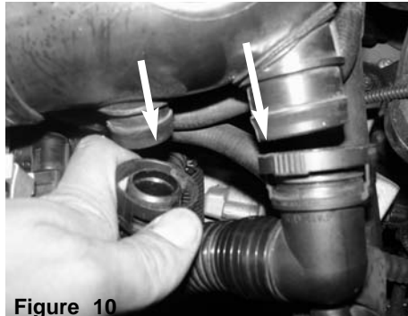
Figure 10 Disconnect the crank case and smog pump fitting clips from stock intake tube. Remove stock intake tube from vehicle.
