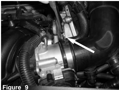
Figure 9 With pliers, pinch remaining clamp on throttle body and pull back towards the intake tube.
