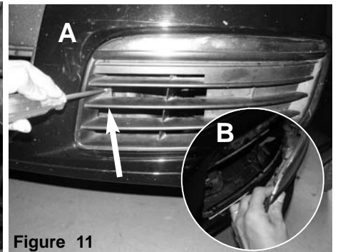
Figure 11 A) With phillips, loosen screw holding in lower bumper valence. B) Pull back and remove valence.
