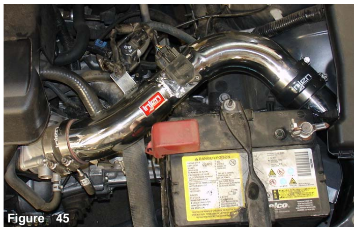
Figure 45 align the entire intake for best possible fit. Once you have established the best fit, free from any moving parts, continue to tighten all nuts, bolts and clamps.
