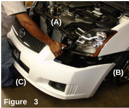
Figure 3 Remove all four clips on top bumper (A), two m6 bolts under the fender well(B), six phillips screws and five clips located under the bumper (C). Now carefully pull the bumper away from the frame.
