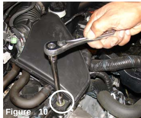
Figure 10 Loosen and remove the m6 bolt located on the CCV box edge.
