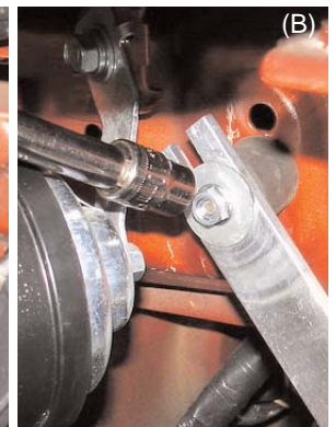
Once the coupler has been pressed into the silicone hose, align the coupler bracket to the vibra-mount stud (A). Place the fender washer and m6 flange nut over the vibra-mount stud and use the 10mm socket to fasten the flange nut to the vibra-mount stud (B).
