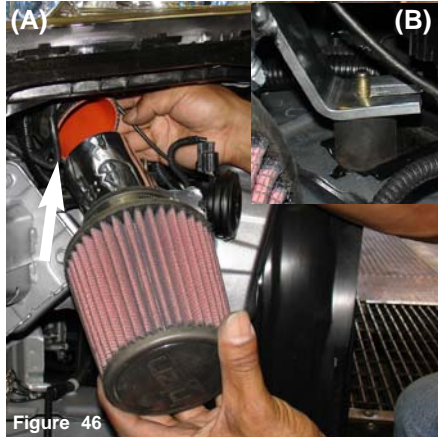
Figure 46 The secondary intake is pressed into the silicone hose (A) and the intake bracket is aligned to the vibra-mount stud(B).
