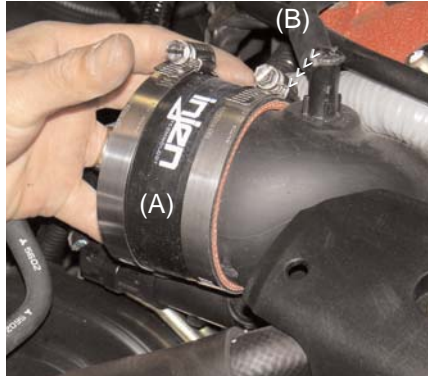
The 3" hose is placed over the air inlet duct and two .362 power-bands are used (A). The clamp on the inlet duct is tightened to prevent the hose from slipping off (B)..
