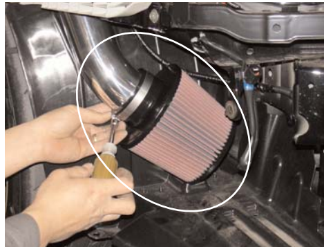
Slip the filter over the end of the intake until it butts up against the stop. Tighten the filter neck clamp to prevent the filter from slipping off.
