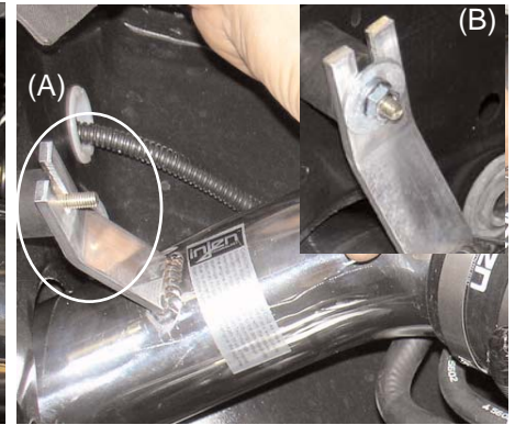
Align intake bracket to the vibra-mount stud (A). Use the m6 flange nut and fender washer to hold the intake in placed (B).
