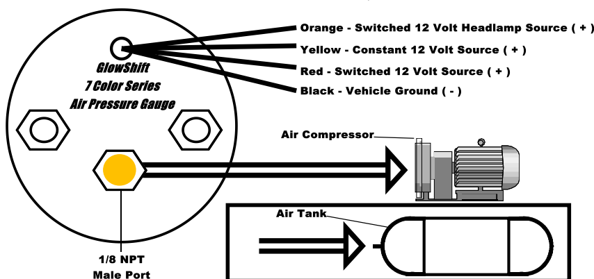
Wire Color Code
