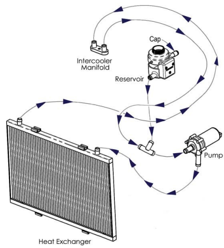
Intercooler Routing Diagram
