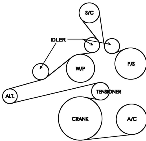
HEMI Belt Routing Diagram
