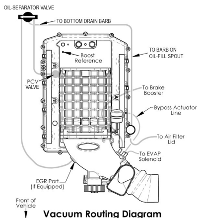
Vacuum Routing Diagram
