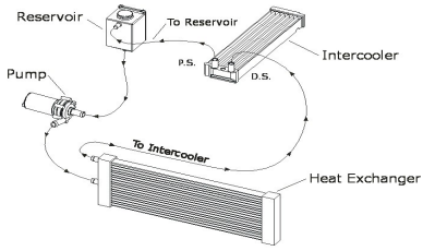
Intercooler plumbing diagram
