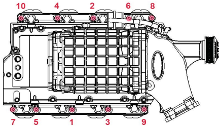
Supercharger Torque Order Diagram
