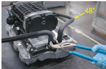
110. Connect the short leg of the cut/assembled 23" x 3" x 3/4" 90° elbow hose to the left hand side charge air cooler hose barb at the back of the supercharger assembly. Secure in place with a provided spring clamp. Connect the cut/assembled 48" x 3" x 3/4" 90° elbow hose to the right hand side charge air cooler hose barb at the back of the supercharger assembly. Secure in place with a provided clamp. The hoses route toward their respective sides as shown.
