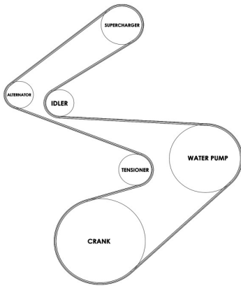
Belt Routing Diagram
