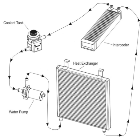
Intercooler Routing Diagram
