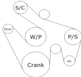
Belt Routing Diagram
