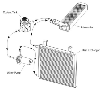
Intercooler Routing Diagram
