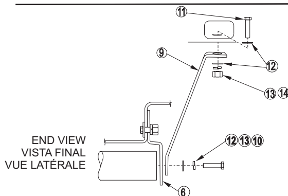
FIGURE 4 DRIVER SIDE SHOWN (REAR BRACE)
