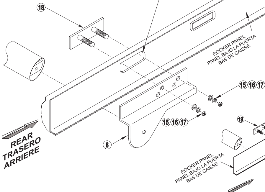
FIGURE 1 DRIVER SIDE REG CAB SHOWN
