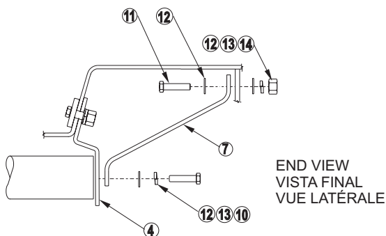
FIGURE 3 DRIVER SIDE SHOWN (FRONT BRACE)
