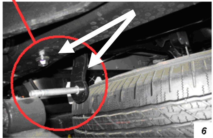
REMOVING REAR OEM SHACKLE ASSEMBLY
