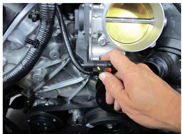
Fig. 1AE: Throttle Body Connector
