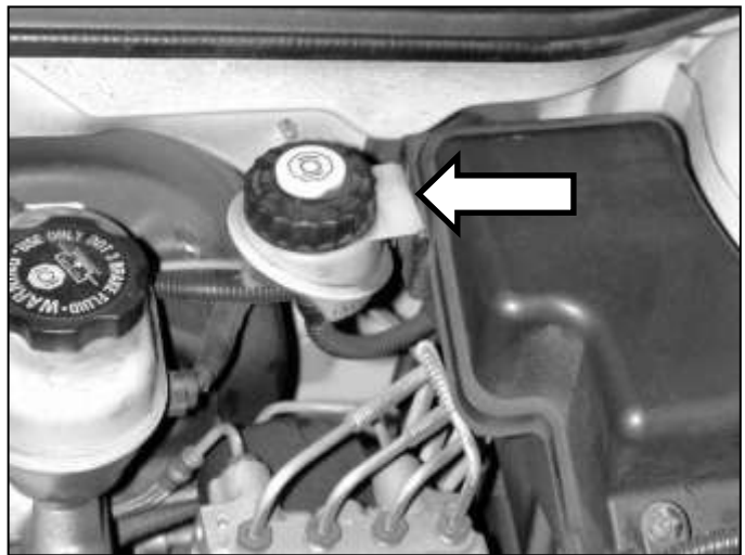
j. If equipped with a manual transmission, remove the clutch fluid reservoir from the air box. Secure it to the firewall with AEM® part # 20-445 (sold separately). Remove the air box from the vehicle.
