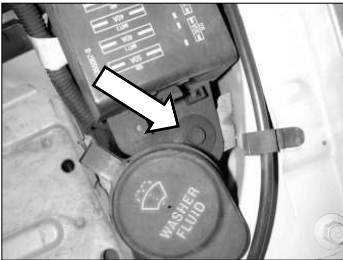
i. Remove the plastic clip that secures the fuse block.
