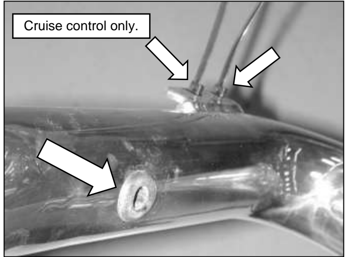
i. Install the supplied grommet in the hole on the upper pipe. Insert the zip tie into the hole on the upper pipe bracket (use two zip ties if the car has cruise control).
