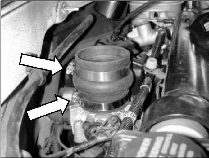
h. Install the hump hose to the throttle body as shown.
