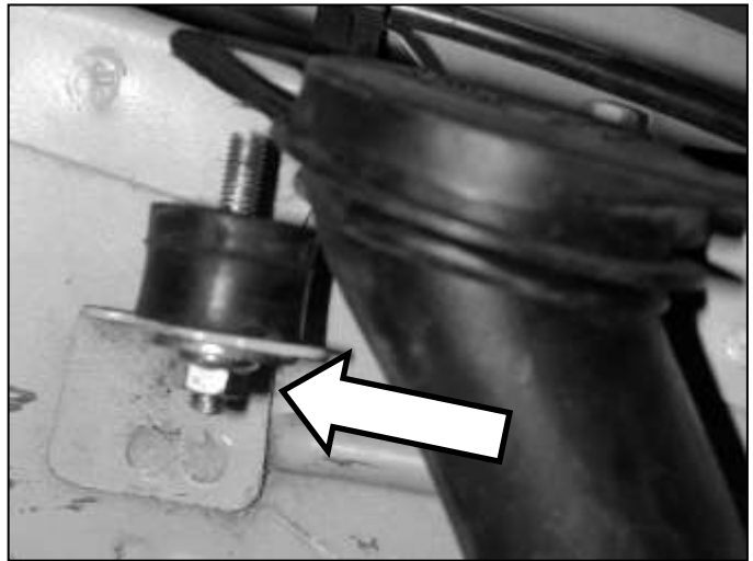
g. Attach the rubber mount to the tab near the washer bottle filler neck using the supplied washer and lock nut.
